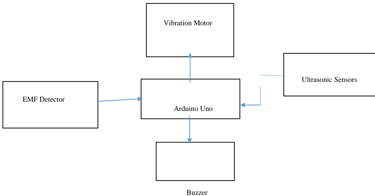
Fig.12: Block diagram of the project
