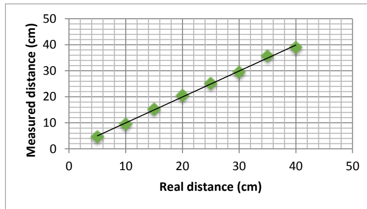
Fig. 15: Relationship between measurement and actual Distance for stone obstacle
