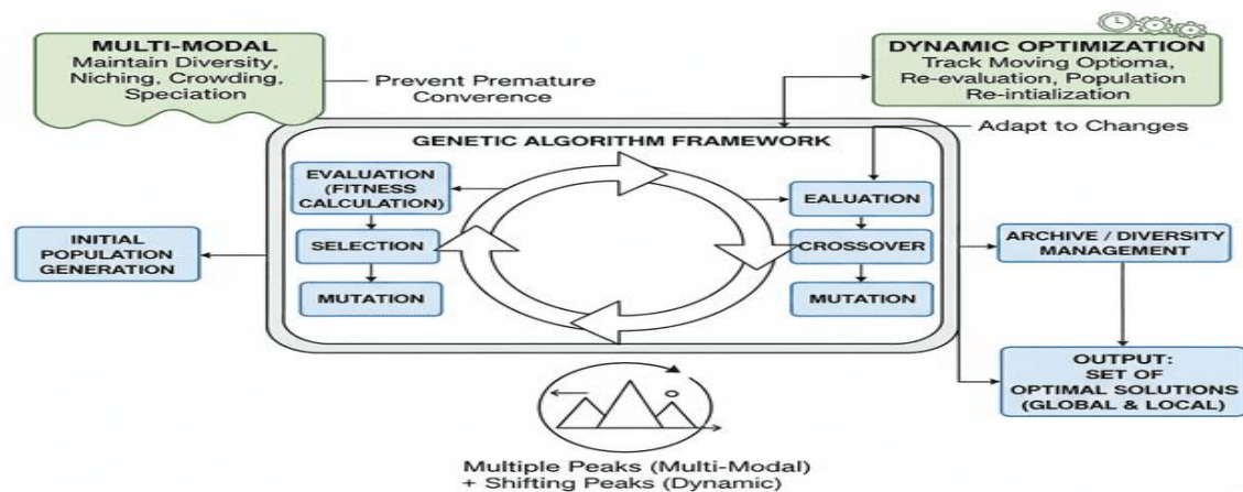
Figure 4: Diagrammatic Representation of Advance Genetic Algorithm Framework Incorporating Strategies for Multi-Modal and Dynamic Optimization (Binsfeld et al., 2025)
